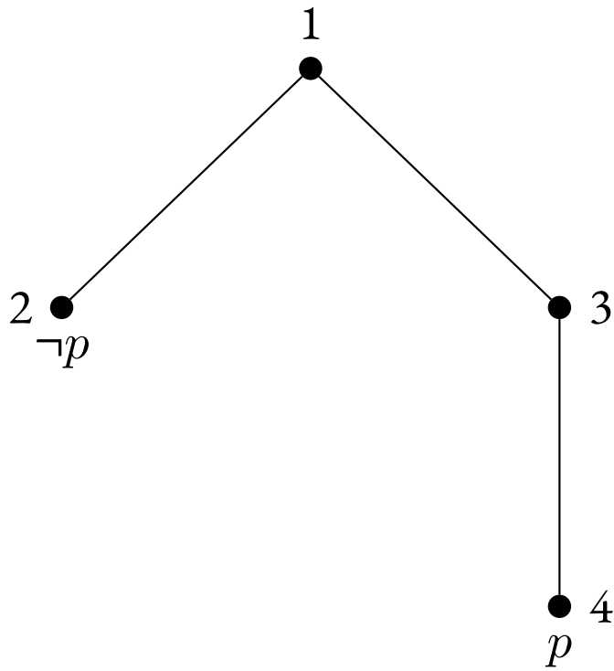
Figure 1: A Kripke Tree to illustrate (P2)
