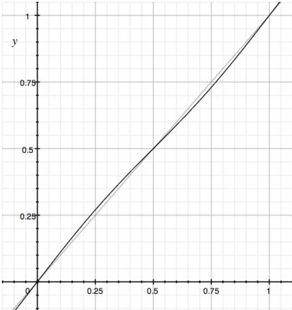
Figure 1: A sine wave around x=y
